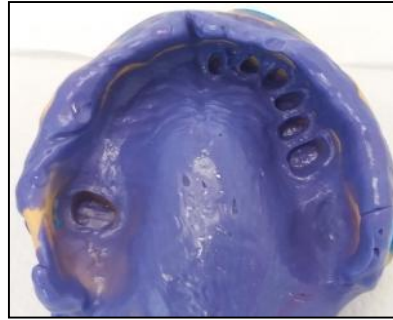
Fig. 6. Maxillary impression
