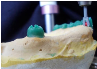
Fig. 9. Fixing the patrice of the attachment
