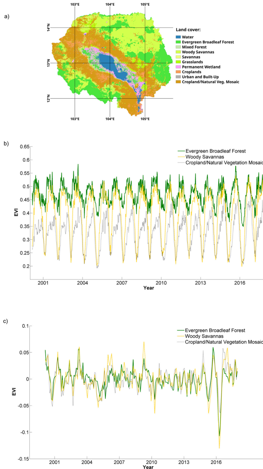
Fig. 8. a) Land cover map of the Tonle Sap watershed from the 500 m MODIS-based Global Land Cover Climatology, b) time series of EVI and c) EVI interannual anomaly averaged over Evergreen Broadleaf Forest (green), Woody Savannas (orange) and Cropland/Natural Vegetation Mosaic (black). (For interpretation of the references to colour in this figure legend, the reader is referred to the web version of this article.)
